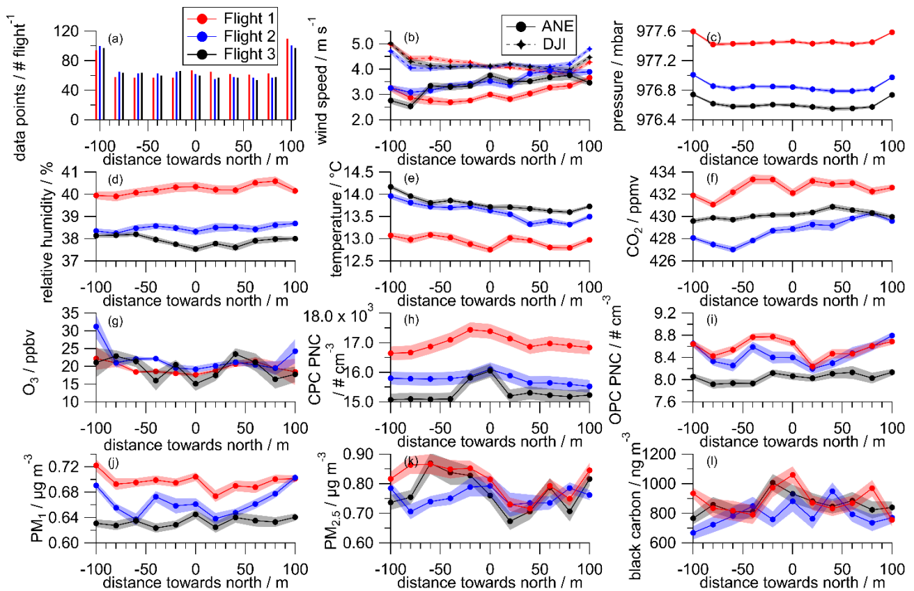
35 Figure S5: Number of data points collected by FLab (a) for horizontal flight 1 (red), flight 2 (blue) and flight 3 (black) with: wind speed determined by ANE (b, dots) and DJI (b, diamonds), pressure (c), relative humidity (d), temperature (e), CO 2 (f) and O 3 mixing ratios (g), CPC and OPC particle number concentrations (h and i), particulate matter PM 1 (j) and PM 2.5 (k) determined from the OPC data, and black carbon mass concentrations (l). The shaded areas indicate the standard error.
