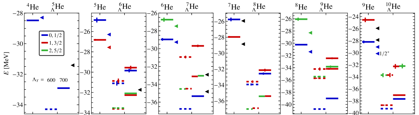
Fig. 2. Extrapolated energies of low-lying natural-parity states of hypernuclei along the helium chain. Shown are the nucleonic parents and the single- \Lambda hypernuclei for two values of the YN interaction regulator \Lambda_Y = 600 MeV/ c (dashed lines) and \Lambda_Y = 700 MeV/ c (solid lines). Experimental values [26,43–47] are marked by triangles, vertical lines denote extrapolation uncertainties. The colors denote angular momenta: blue for J = 0 ( 1/2 ), red for J = 1 ( 3/2 ), and green for J = 2 ( 5/2 ) for even (odd) systems. Unknown angular momenta are marked by black symbols.
