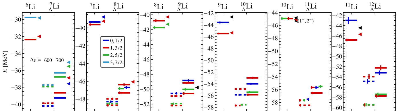
Fig. 4. Like Fig. 2, but for the lithium chain. The colors denote angular momenta: blue for J = 0 ( 1/2 ), red for J = 1 ( 3/2 ), green for J = 2 ( 5/2 ) and light blue for J = 3 ( 7/2 ) for even (odd) systems. Unknown angular momenta are marked by black symbols. Experimental values are taken from [26,43–46,48].
