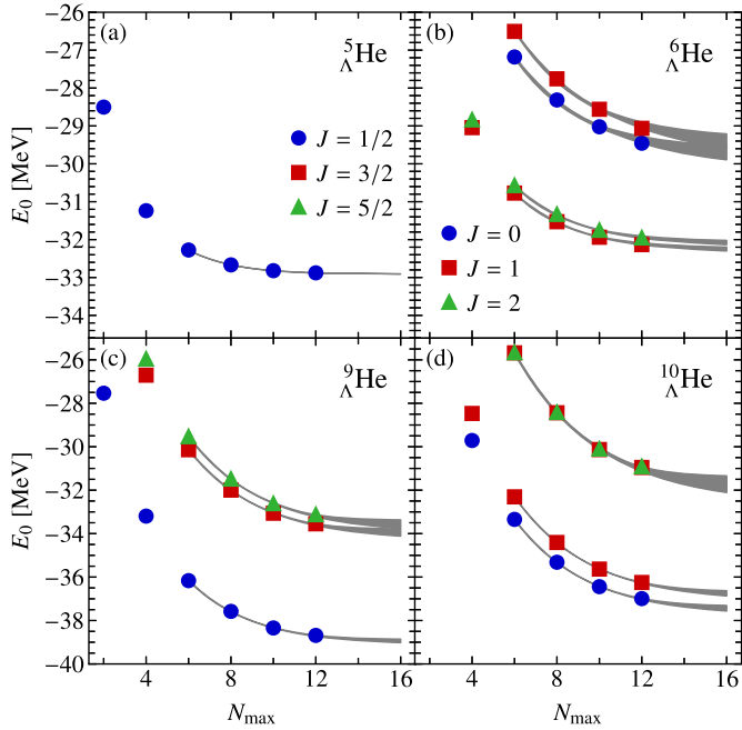
Fig. 1. Absolute energies of the low-lying spectrum of four helium hypernuclei for the YN interaction with \Lambda_Y = 700 MeV/ c cutoff. The colors denote angular momenta: blue for J = 0 ( 1/2 ), red for J = 1 ( 3/2 ), green for J = 2 ( 5/2 ) for even (odd) systems. The gray bands mark the envelope of the fit functions used to extrapolate the energies to infinite model-space size. Note that the nuclei shown in (a) and (c) are particle-stable while those in (b) and (d) are not, according to the calculation. (For interpretation of the colors in the figure(s), the reader is referred to the web version of this article.)
