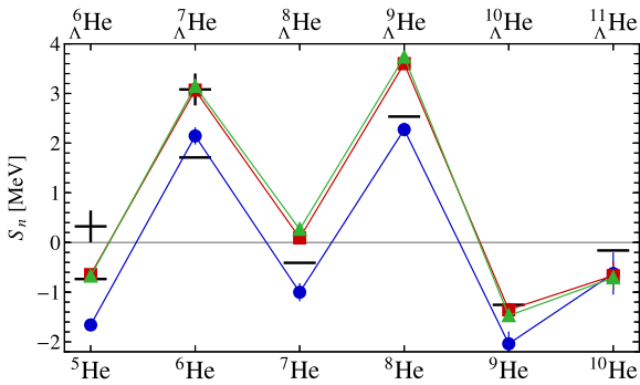
Fig. 3. Neutron separation energies of helium (hyper-)isotopes. Shown are the separation energies calculated for the nucleonic parents (blue circles) and for their daughter hypernuclei using the \Lambda_Y = 700 MeV/c (red squares) and \Lambda_Y = 600 MeV/c (green triangles) cutoffs. Experimental values are shown as black bars (crosses) for the (hyper-)nuclei. Vertical lines indicate extrapolation uncertainties.
