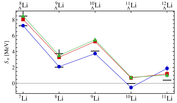
Fig. 5. Same as Fig. 3, but for lithium (hyper-)isotopes.
