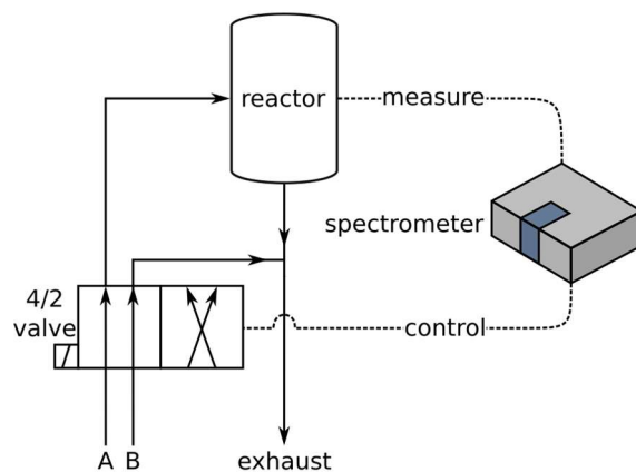
Figure 1: Scheme of the experimental ME-DRIFTS setup. For details see text.
