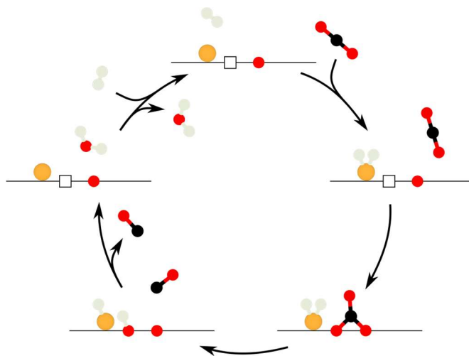
Figure 4: Proposed mechanism for the RWGSR over Au/CeO 2 based on the presented ME-DRIFTS results.
