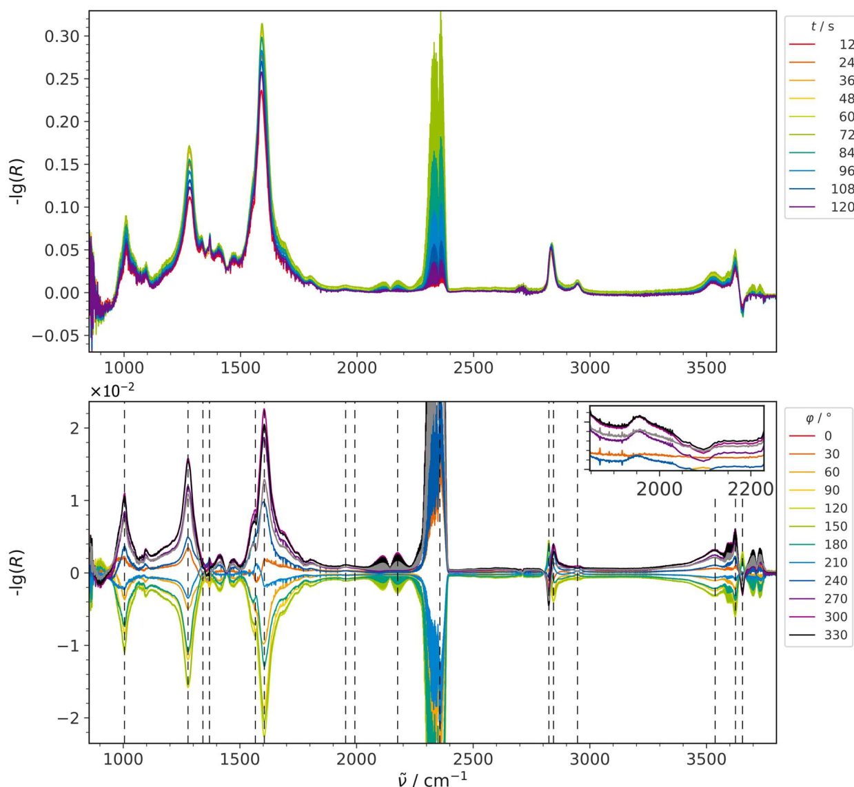
Figure 2: ME-DRIFT spectra during RWGSR over Au/CeO 2 for CO 2 modulation conditions, that is, switching the CO 2 concentration between 0 and 2 mol%, while keeping the H 2 concentration constant at 4 mol%. Top: Selected spectra from the time-resolved data set before applying PSD. Bottom: PSD spectra in an enlarged view cutting the intensity of the gas-phase CO 2 signal. The inset provides an enlarged view of the Au-H 2 signal. Signal positions from Tab. 1 are indicated by dashed lines.
