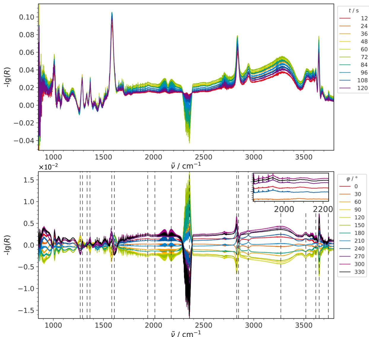
Figure 3: ME-DRIFT spectra during RWGSR over Au/CeO 2 for CO 2 modulation conditions, that is, switching the H 2 concentration between 0 and 4 mol%, while keeping the CO 2 concentration constant at 2 mol%. Top: Selected spectra from the time-resolved data set before applying PSD. Bottom: PSD spectra. The inset provides an enlarged view of the Au-H 2 signal. Signal positions from Tab. 2 are indicated by dashed lines.
