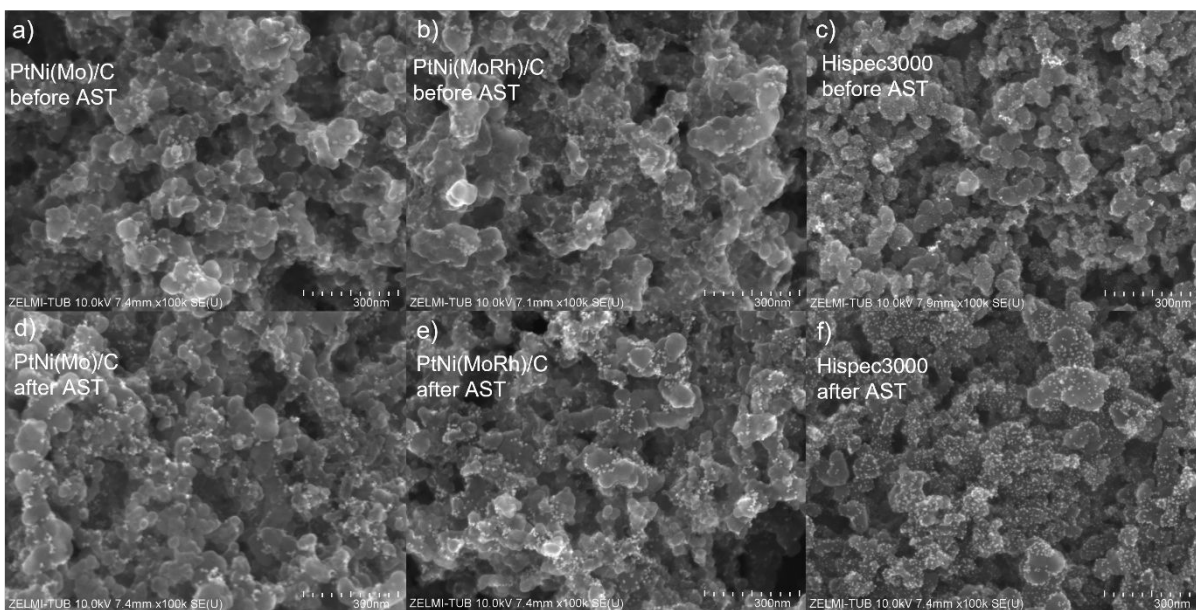
Figure S20: SEM images of PtNi(Mo)/C, PtNi(MoRh)/C, and Hispec3000 a) – c) before AST and d) – f) after AST with a magnification of 100k.
