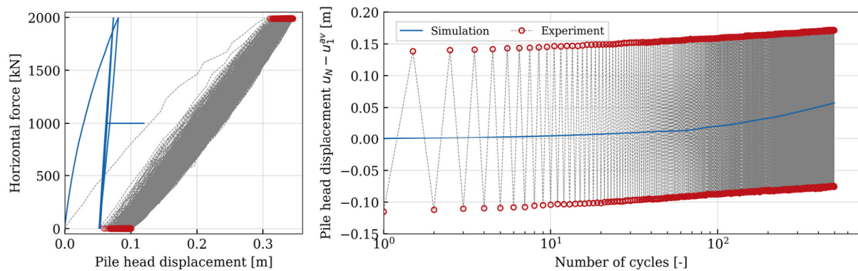
Fig. 10. Comparison between experiment and simulation of the cyclically loaded pile group: horizontal force at the pile head vs. pile head displacements (left); Pile head displacement vs. number of load cycles (right). Here, pile head refers to the load application point of the pile group (cf. Fig. 7). The red circles represent the pile head displacements measured at maximum and minimum load level of each cycle. The deformations from the cyclic loading are given relative to the deformation of the first irregular cycle measured at average load H_{av} .
