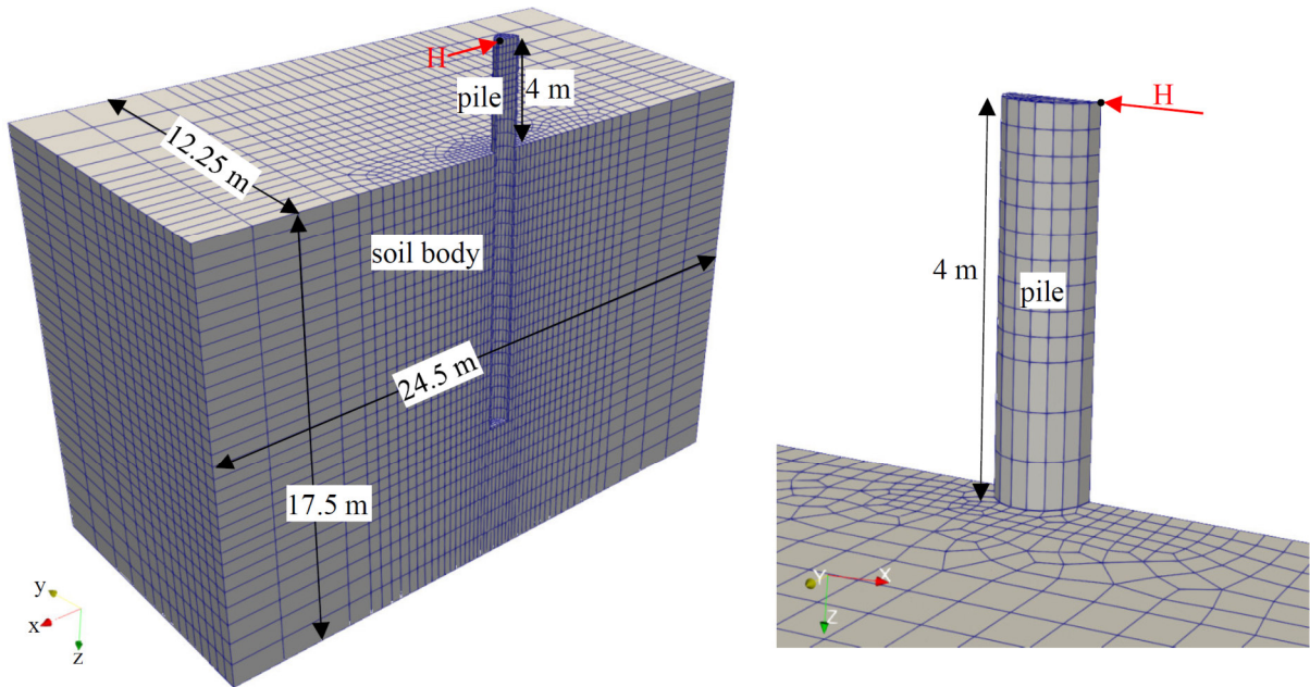
Fig. 6. Finite element model of the single pile (exploiting symmetry).
