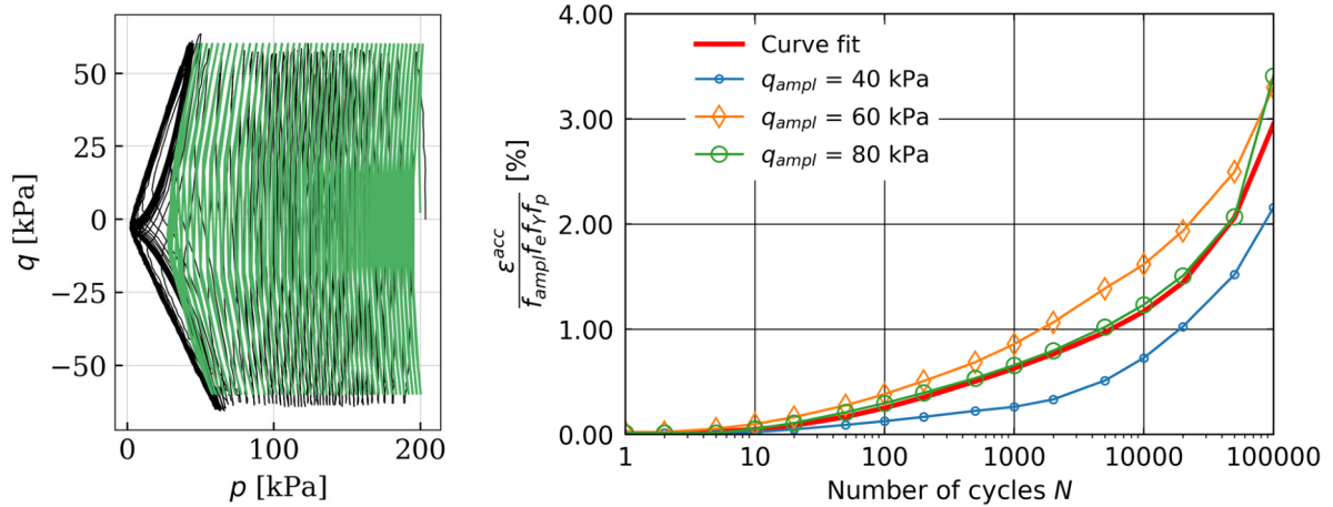
Fig. 5. Left: Comparison of simulation (green) and test result (black) of one undrained cyclic triaxial test. Right: Strain accumulation divided by the functions f_{amp} , f_e , f_y and f_p of the HCA model versus number of applied load cycles for three drained high-cyclic triaxial tests with different stress amplitude. The plots are curve-fitted in order to obtain the parameters C_{N1} , C_{N2} and C_{N3} .
