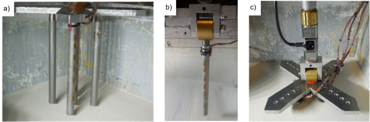
Fig. 2. Experimental setup of the pile tests: a) pile group before installation, b) single pile before installation, c) installed pile group with hinge and load cell (after Niemann 2020).
