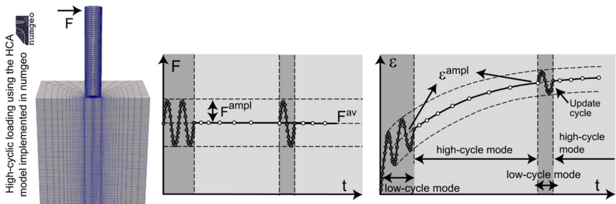
Fig. 3. FE simulation of high-cyclic loading using a combination of low-cycle and high-cycle calculation phases (after Staubach et al. 2021).
