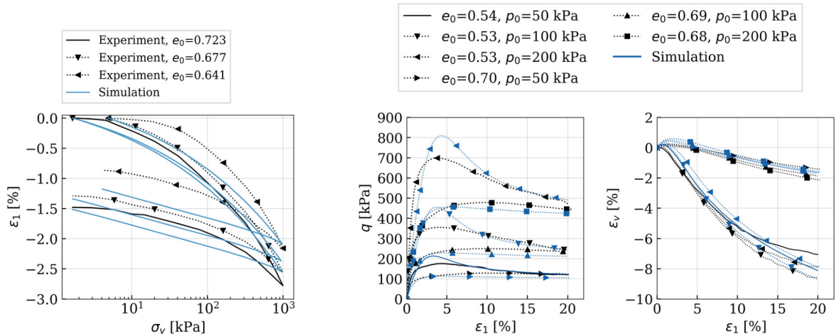
Fig. 4. Comparison of simulations (blue lines) and test results (black lines) of oedometric compression tests (left) and drained monotonic triaxial tests (right) on samples with different initial densities and different initial mean effective stresses.
