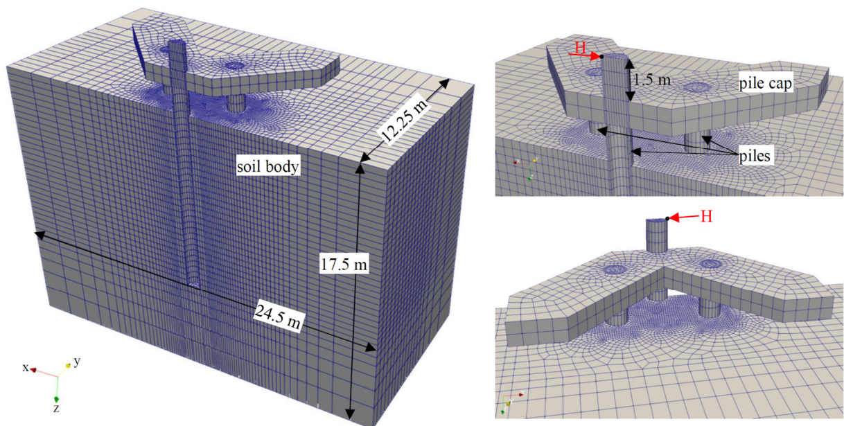
Fig. 7. Finite element model of the pile group (exploiting symmetry).
