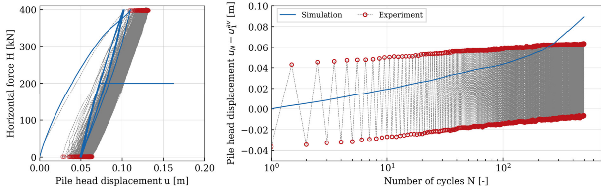
Fig. 9. Comparison of experiment and simulation for the cyclically loaded single pile: horizontal force at pile head vs. pile head displacement (left); Pile head displacement vs. number of load cycles (right). The red circles represent the pile head displacements measured at maximum and minimum load level of each cycle. The deformations from the cyclic loading are given relative to the deformation of the first irregular cycle measured at average load H_{av} .
