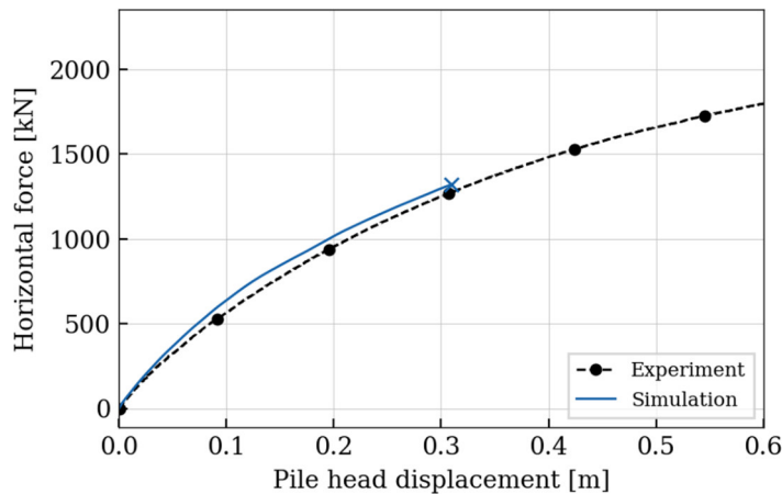
Fig. 8. Comparison of horizontal force at pile head vs. pile head displacement of the monotonic single pile test for experiment (dotted line, black) and simulation (solid line, blue).
