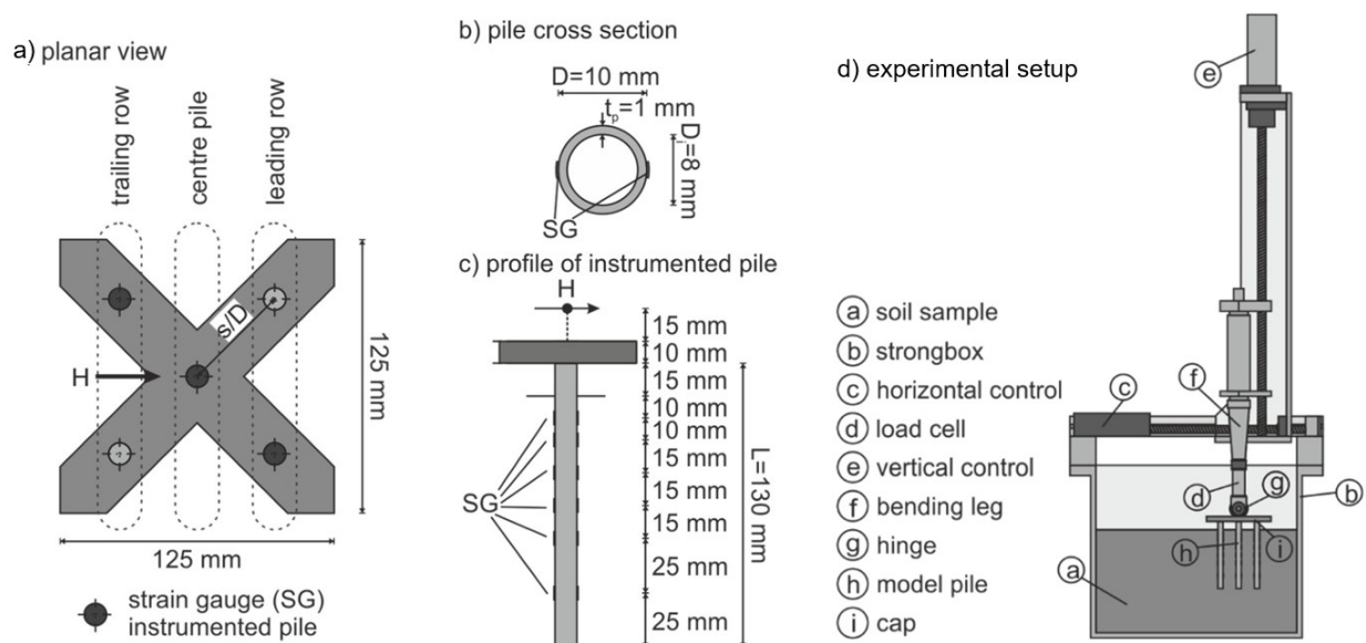
Fig. 1. Centrifuge tests: Pile group geometry in model scale, instrumentation and experimental setup (after Niemann 2020).
