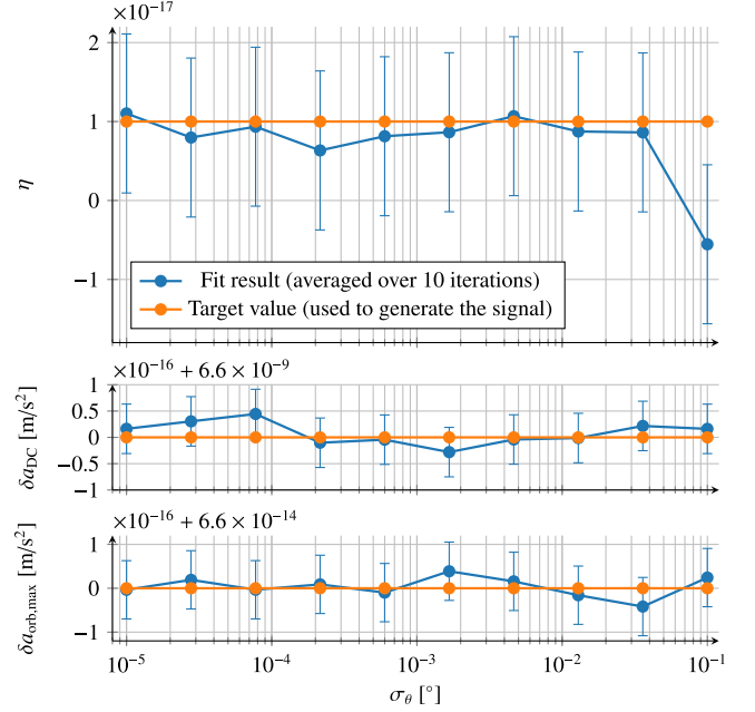
FIG. 6. Attitude control analysis. The signal was generated using Eq. (32) for \eta = 10^{-17} , \delta a_{\text{DC}} = 6.6 \times 10^{-9} m/s 2 , and \delta a_{\text{orb,max}} = 6.6 \times 10^{-14} m/s 2 . Each row displays the fit result for the respective parameter that is shown for various attitude noise levels \sigma_{\Delta\theta} . The orange points show the target values, whereas the blue points show the recovered value from the fit. The error bars represent the standard deviation of the ten fits.
