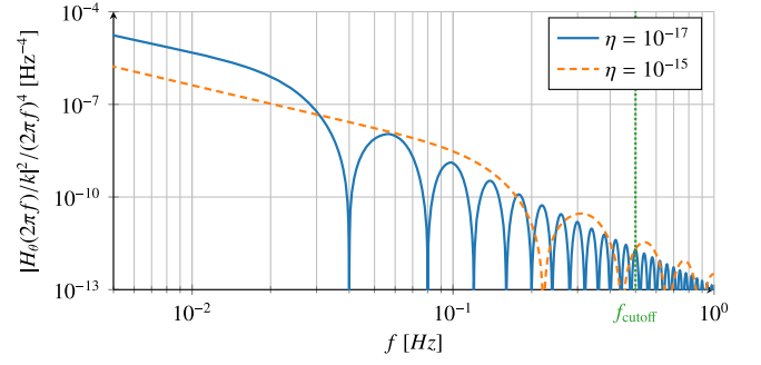
FIG. 4. Angular acceleration transfer function, Eq. (25), using the parameters in Table I. For low frequencies f \ll 2/T it behaves as f^{-1} while for larger frequencies f \gg 2/T it follows f^{-2} , similar to the linear acceleration transfer function (see Fig. 2). The frequency cutoff f_{\text{cutoff}} up to which the integration in Eq. (26) is performed is marked in dotted green.
