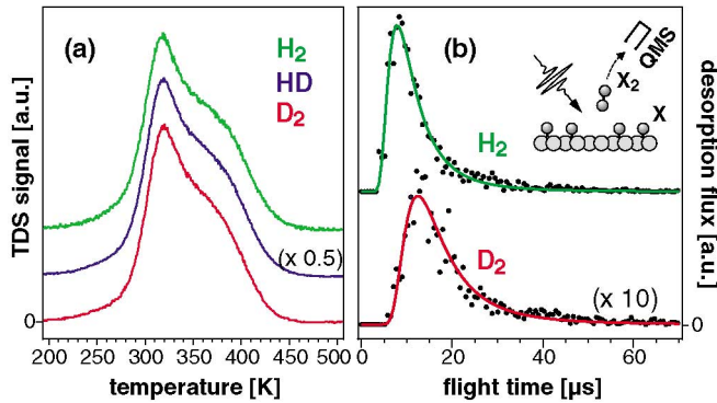
FIG. 1 (color). (a) TD spectra for H_2 , HD, and D_2 from a saturation coverage of HD. Spectra are scaled according to detection sensitivity and offset for clarity. (b) The fs-laser induced TOF spectra for H_2 (offset) and D_2 . Mean kinetic energies are obtained by fitting modified Maxwell-Boltzmann distributions (solid lines) to the experimental data. E_{kin} = (2110 \pm 400) K and (1720 \pm 290) K for H_2 and D_2 , respectively.
