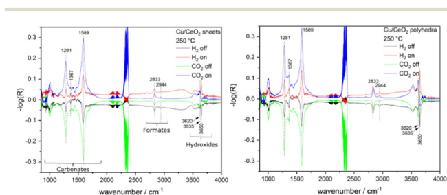
Fig. 3 Transient DRIFT spectra of Cu/CeO 2 sheets (left) and polyhedra (right). The spectra were recorded after pretreatment in H 2 , CO 2 or H 2 /CO 2 balanced in argon at 250 °C at a total gas flow of 100 ml min -1 . Prior to the measurements, the H 2 (CO 2 ) supply was switched on while CO 2 (H 2 ) remained constant or the H 2 (CO 2 ) was switched off while the CO 2 (H 2 ) remained constant. Shown are only the last spectra of a measurement series recorded after 12 min. For details see SI†
