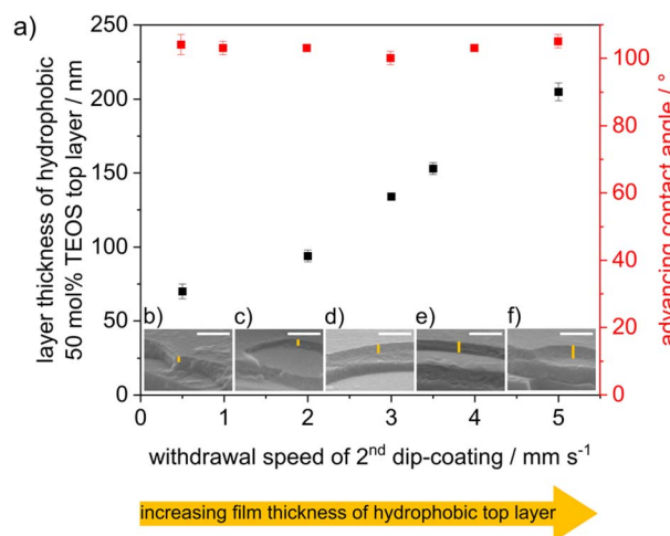
Fig. 5 (a) Thickness of the top layer (black) determined by ellipsometry and advancing water contact angle (red) of mesoporous silica film consisting of a hydrophilic bottom layer and a hydrophobic top layer and dependence of the withdrawal speed, while dip-coating of the second layer. (b–f) SEM images of double layer silica film using different withdrawal speeds of dip-coating of the second layer. Scale bar (SEM): 500 nm.
