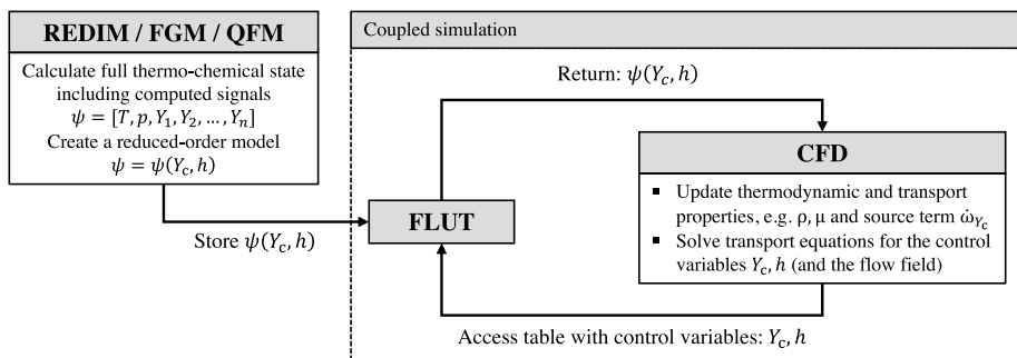
Fig. 1 Illustration of the look-up procedure of a coupled simulation using chemistry manifolds. The full thermo-chemical state is estimated by the chemistry manifold including computed signals and incorporated into a FLUT. During the coupled simulation, the transport equations of the control parameters are solved and the thermodynamic and transport properties are updated by a table look-up during runtime
