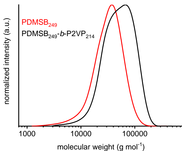
Figure S8: Molecular weight distribution of PDMSB 249 - b -P2VP 214 (52.3 vol% PDMSB) and the corresponding PDMSB aliquot according to SEC measurements in THF against polystyrene standards.
