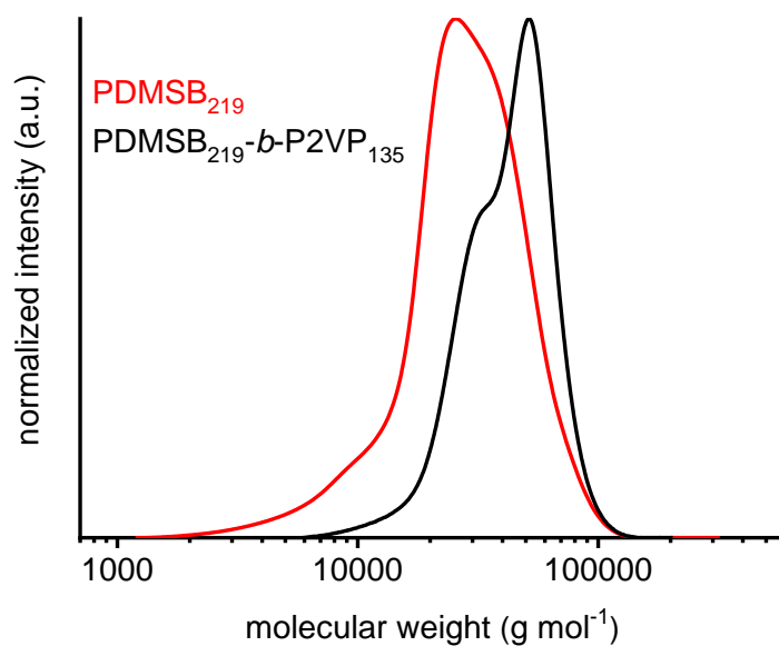
Figure S9: Molecular weight distribution of PDMSB 219 - b -P2VP 135 (60.5 vol% PDMSB) and the corresponding PDMSB aliquot according to SEC measurements in THF against polystyrene standards.
