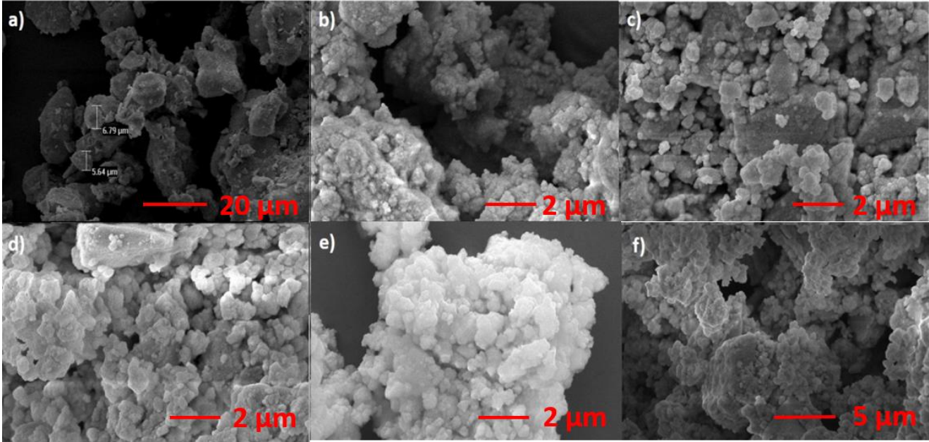
Fig. S1: SEM micrographs recorded for the a) as synthesized LLZTO powders. Powders milled at 600 RPM for b) 4 Hours c) 8 hours, d) 12 hours, e) 16 hours and f) 20 hours.
