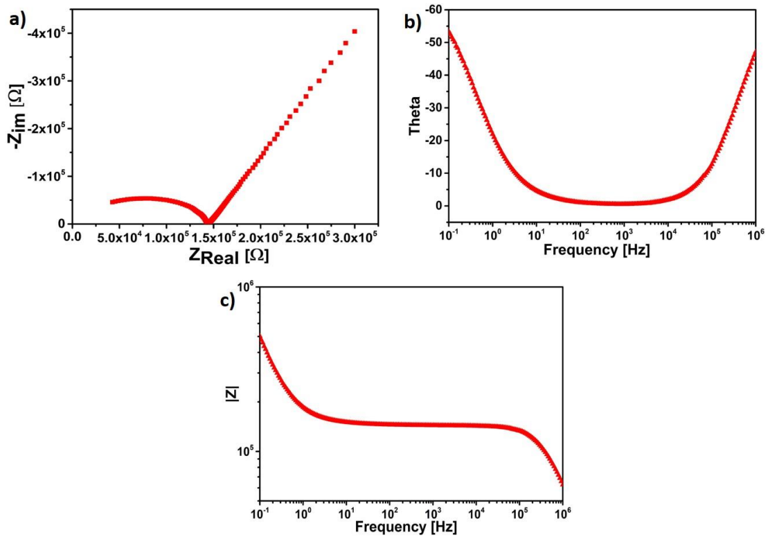
Fig. S2:-NYQUIST and Respective bode plot measured for PEO with molecular weight 100000 with 1:30 molar ratio of LiTFSI.
