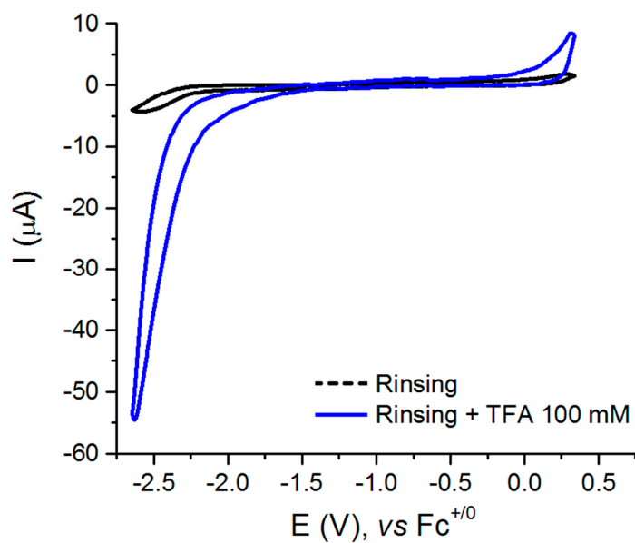
Figure S20. Cyclic voltammograms recorded after electrocatalysis of \text{Ni}_3\text{L}_2 upon washing the working electrode and immersion into a fresh solution of dry DMF (0.1M \text{NBu}_4\text{PF}_6 , black dashed line) and in the presence of 100 mM of TFA (blue line). Scan rate 500 \text{ mV s}^{-1} .
