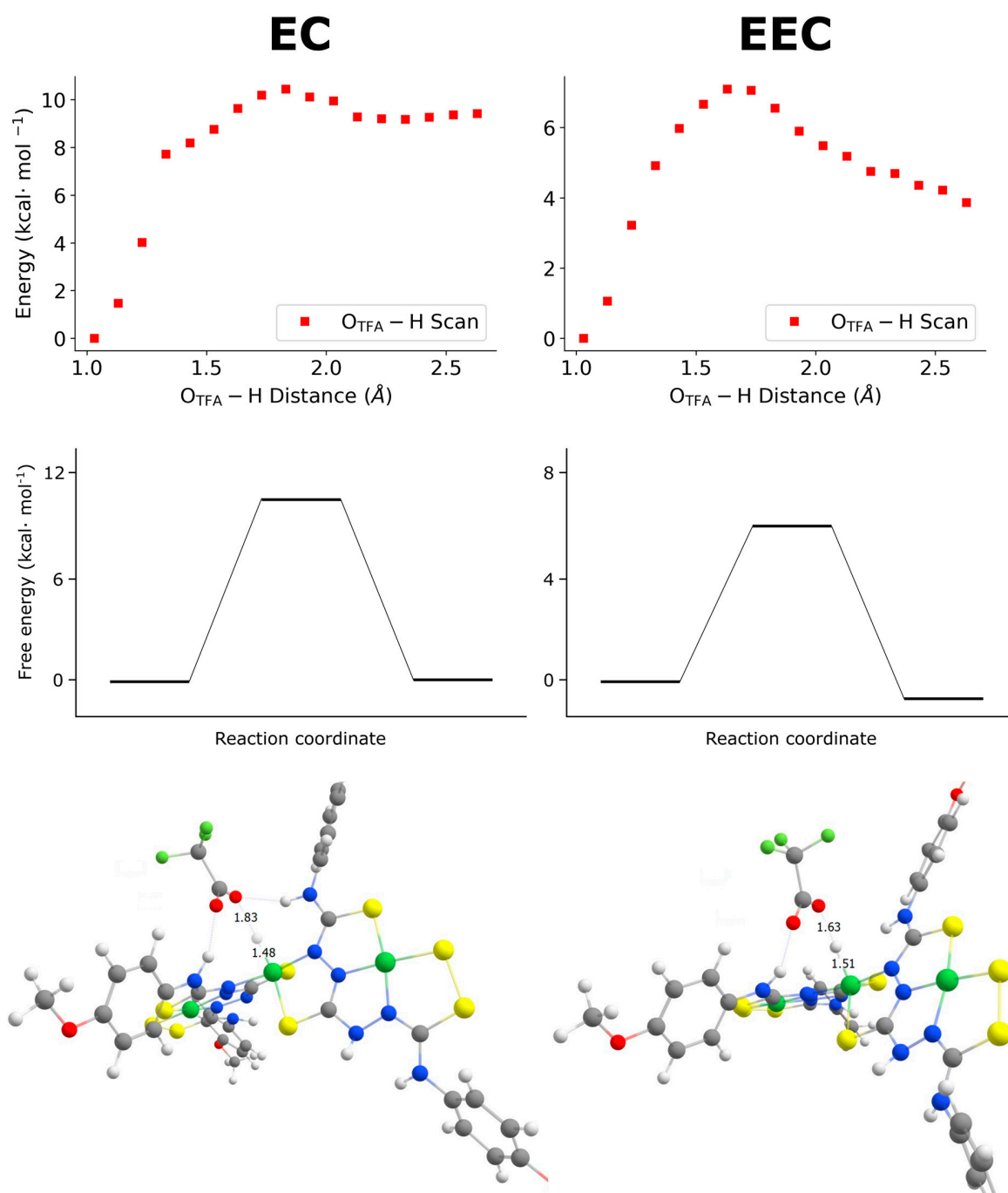
Figure S27. Potential energy surface scans for the proton transfer between TFAH and \text{Ni}_3\text{L}_2 after the first (left) and second (right) reductions (top), free energy diagrams of the proton transfer, where the transition state was taken as the highest point in the PES scan (middle) and transition state geometries, with Ni-H and \text{O}_{\text{TFA}}\text{-H} distances displayed in Å (bottom). Their cartesian coordinates are provided in Tables S14 and S15.
