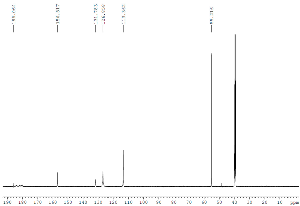
Figure S4. ^{13}\text{C} NMR spectrum and partial assignment for \text{H}_6\text{L} in DMSO at 298 K.
