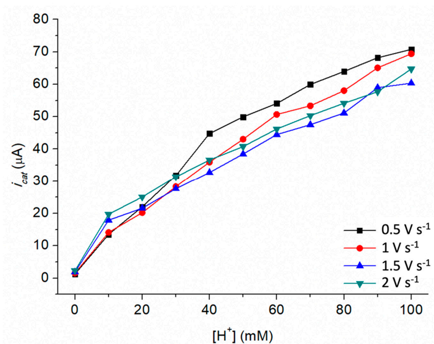
Figure S19. Plot of i_{cat} of \text{Ni}_3\text{L}_2 for increasing concentrations of TFA at different scan rates.
