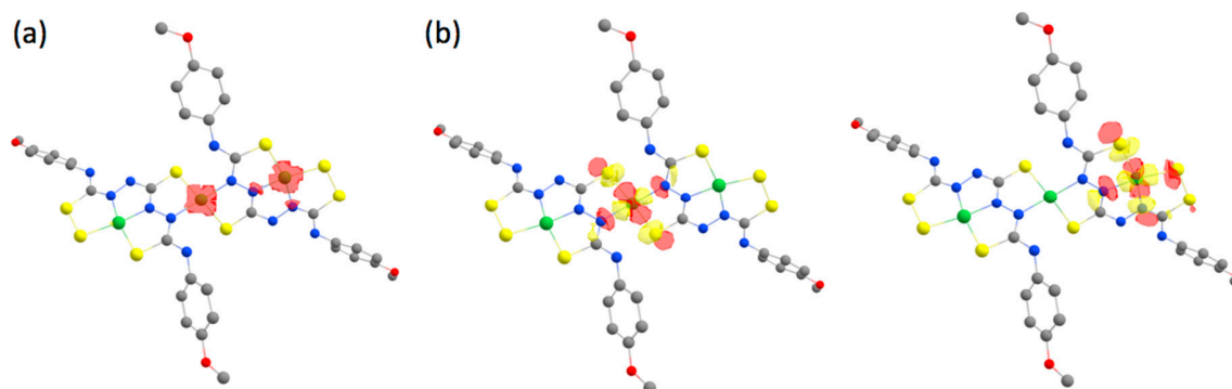
Supplementary figure S26. Spin density plot (a) and localized Singly Occupied Molecular Orbital (SOMO, b) for \text{Ni}_3\text{L}_2 after two subsequent one-electron reduction reactions. The complex is in a triplet dianionic state.
