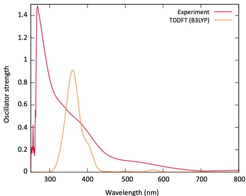
Figure S10. Comparison between experimental and calculated UV-Vis spectra for \text{Ni}_3\text{L}_2 in DMF. Calculations performed on the neutral complex in a closed-shell singlet state (B3LYP/def2-TZVP(-f), see Electronic structure section in the main text).
