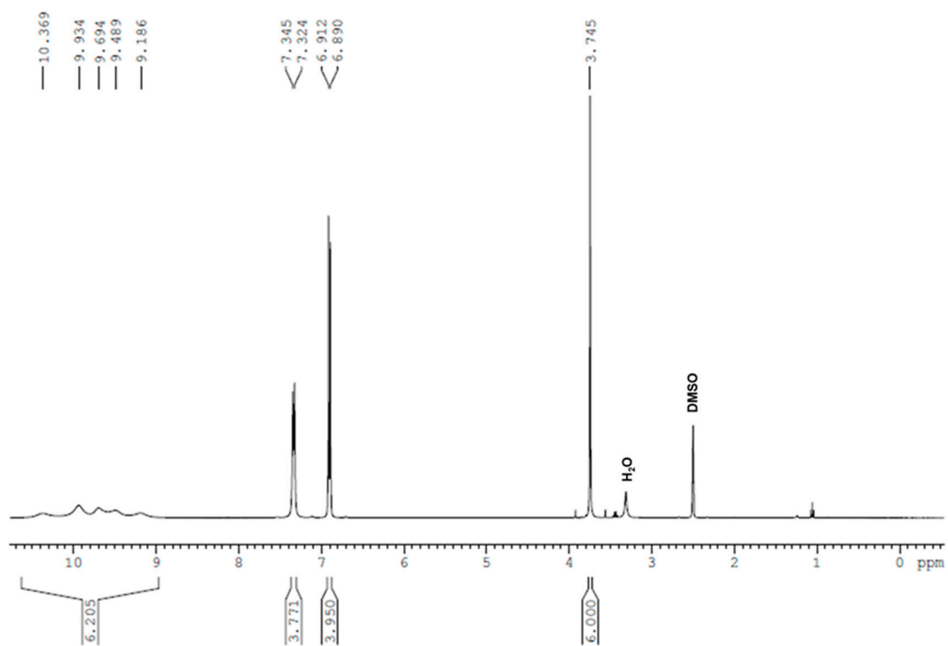
Figure S3. ^1\text{H} NMR spectrum and partial assignment for \text{H}_6\text{L} in DMSO at 298 K.
