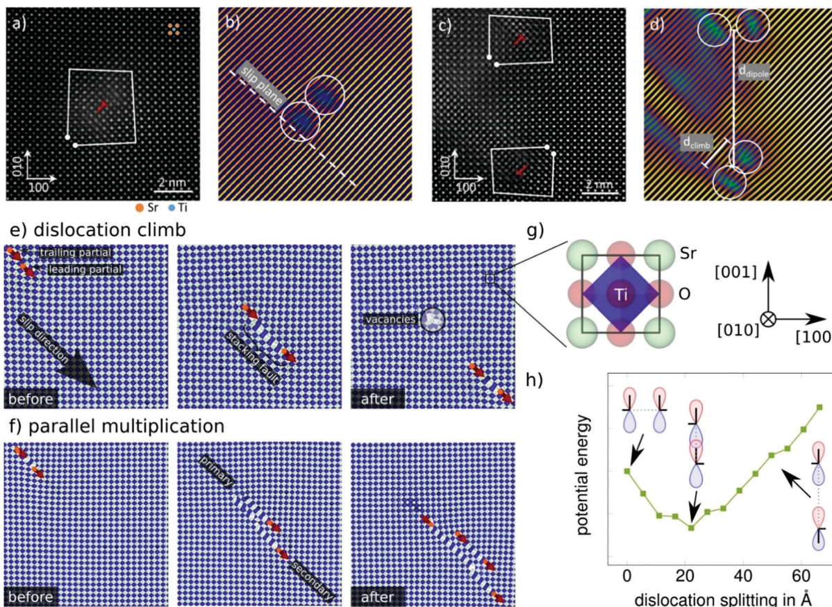
Fig. 2 Dislocation structure at atomic resolution. (a) HAADF image of the dislocation core of a \{110\}\{110\} type dislocation with Burgers circuit. (b) Atom planes corresponding to (a), illustrating that the partial dislocations have climb-dissociated (see supplementary 10, ESI † ), likely due to the electron beam. (c) Dislocations in close vicinity with less than 15 unit cells distance revealing opposite line vectors. (d) Atom planes corresponding to (c). (e) Molecular dynamics simulations highlight spontaneous climb of a dislocation and creation of a defective region with vacancies. Dislocation lines are indicated in orange and the direction of the Burgers vector as red arrow. (f) One of two dislocation partials climbs to a parallel (secondary) glide plane while the other stays on its original (primary) plane. New partials spawn to complete the singular partials. On the lower plane an extended stacking fault is created between the partials which is relieved by creating further partial dislocations effectively multiplying the dislocation. (g) Representation of a \text{SrTiO}_3 unit cell. The blue shapes represent polyhedra of oxygen around titanium and are well suited to identify defects such as stacking faults. For clarity the oxygen atoms are not shown in (e) and (f). (h) Dependence of the energy of two partial dislocations on their separation distance in climb dissociation. Partial dislocations of the shown type have a tendency to climb, see (a–d) as well as (e) and (f), which is energetically favored over dissociation in slip direction. For full details see Supplementary 12 (ESI † ). (a–d) reprinted with permission from Porz, et al. , ACS Nano , DOI: 10.1021/acsnano.0c04491. Copyright (2020) American Chemical Society.
