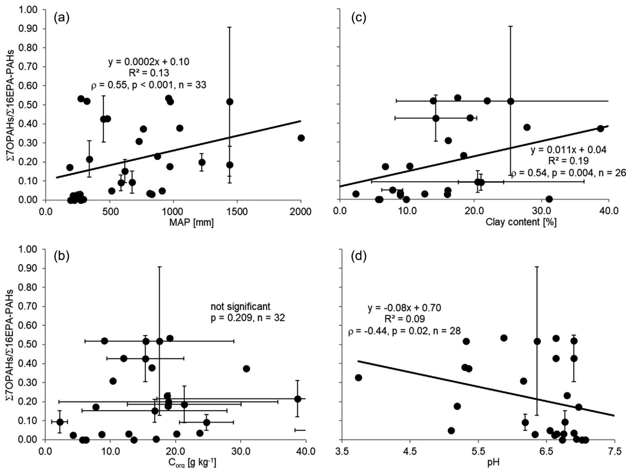
FIGURE 4 Relationship of (a) mean annual precipitation (MAP), (b) organic C concentrations ( C_{org} ), (c) clay contents, and (d) pH with the \Sigma 7\text{OPAH}/\Sigma 16\text{EPA-PAH} concentration ratios. The results of the sites with the same climate were averaged. Error bars show SD
