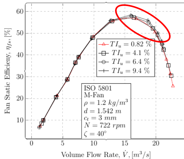
Figure 13: Fan static efficiency at various turbulence intensities.
