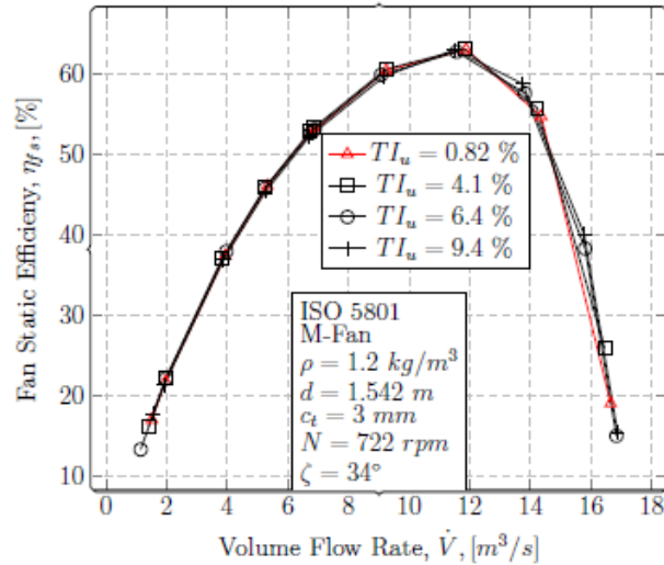
Figure 10: Fan static efficiency at various turbulence intensities.
