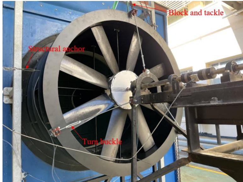
Figure 4: Structural mounting of the annular duct.
