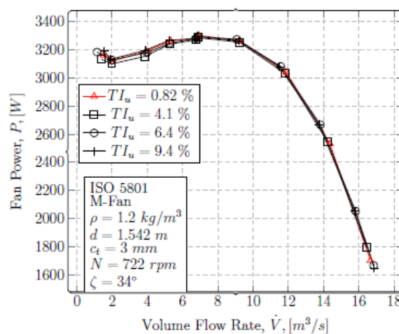
Figure 9: Fan power at various turbulence intensities.
