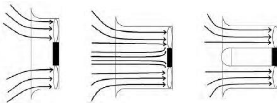
Figure 5: Free inlet (left), ducted inlet (center) and annular inlet (right).
