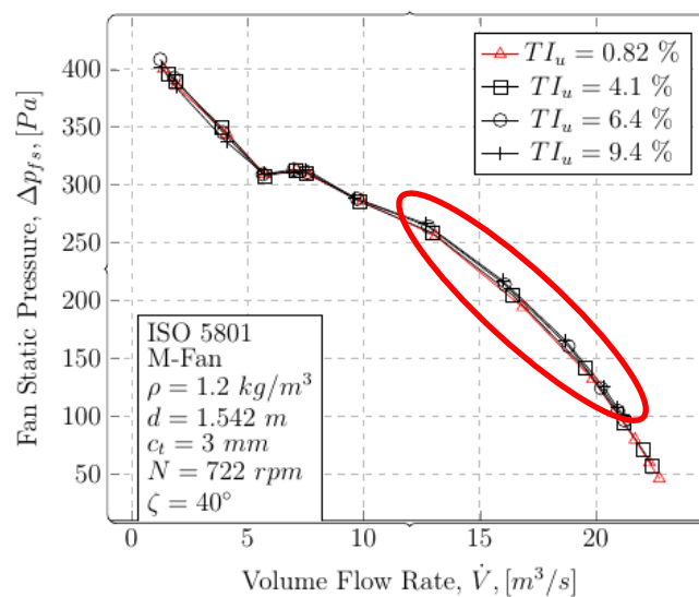
Figure 11: Fan static pressure at various turbulence intensities.
