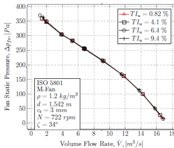
Figure 8: Fan static pressure at various turbulence intensities.
