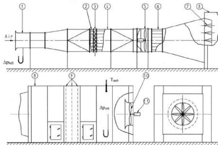
Figure 3: ISO 5801 Type A fan test facility [8].
