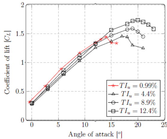
Figure 1: NASA LS 0413 Coefficient of lift at Re = 620 000.
