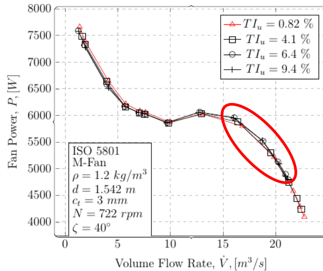
Figure 12: Fan power at various turbulence intensities.
