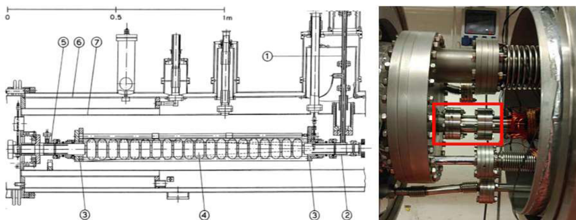
Figure 1. Technical drawing of one half S-DALINAC cryomodule (left picture) [9]. The cavities (3), the couplers (2,5) and the frequency tuners (4) are sitting inside the helium vessel (7) on an aluminium bench. The helium vessel is hanging on the 80 K shield (6) by steel rods. The 500 W rf power is coupled in by a coaxial line (1). On the right picture the interconnection in between two modules is shown [11]. The big bellow of the helium gas return line is relatively stiff and can induce stress in between helium vessels from different modules. The beam tube is located in the red box.
