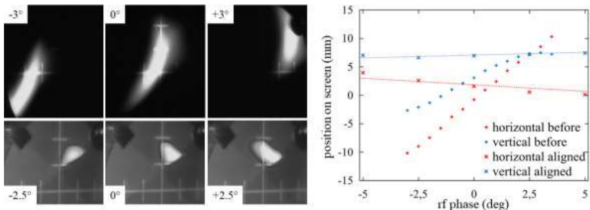
Figure 2. Deflection of the beam on a scintillating BeO screen 5.3 m downstream when changing the rf phase of the 5-cell capture cavity with respect to the optimum ( 0^\circ ). The tics on the target cross axis are 5 mm apart. Before correction (upper series) the beam is steered over the complete target. Proper focusing was impossible. After correction (lower series) the beam is much less steered and focused much better at the optimum rf phase. A total change of rf phase of more than 20 deg was possible without losing the beam on the screen
