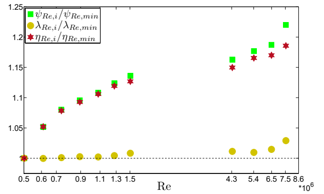
Figure 12. SPLIT-UP OF EFFICIENCY INCREASE ON POWER AND PRESSURE COEFFICIENT
