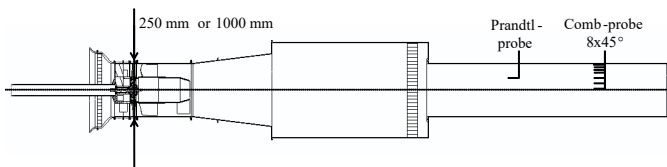
Figure 1. MEASURING POSITIONS FOR DETERMINING THE VOLUME FLOW RATE
