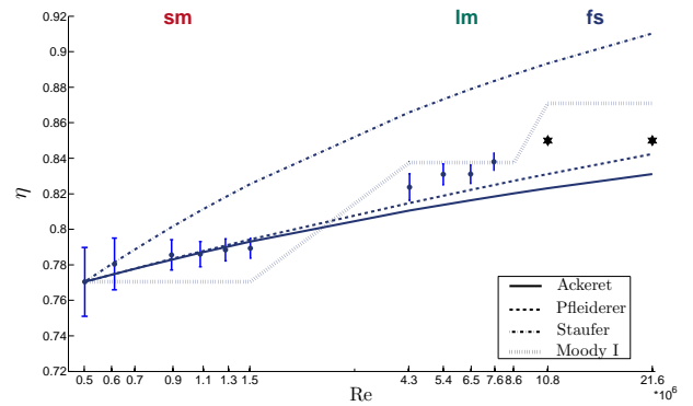
Figure 9. SCALE-UP AT \varphi/\varphi_{opt} = 0.9, \Delta\beta_s = 0^\circ
