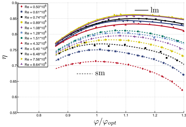
Figure 4. INCREASE OF EFFICIENCY FOR DIFFERENT REYNOLDS-NUMBERS AND \varphi/\varphi_{opt} at \Delta\beta_s = -6^\circ
