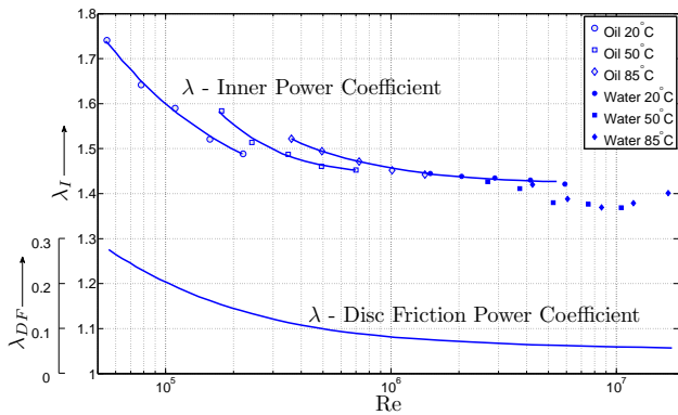
Figure 11. MEASURED INNER POWER COEFFICIENT \lambda_I AND CALCULATED DISC FRICTION POWER COEFFICIENT \lambda_{DF} AS FUNCTION OF REYNOLDS-NUMBER [8]
