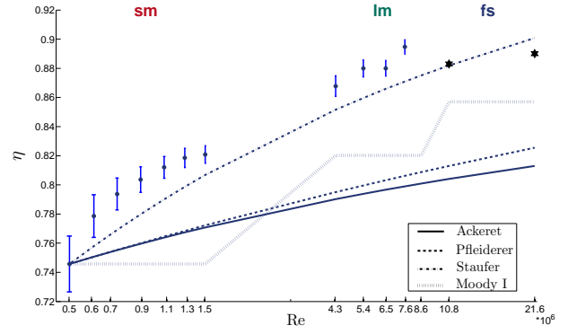
Figure 8. SCALE-UP AT \varphi/\varphi_{opt} = 1.2, \Delta\beta_s = 0^\circ
