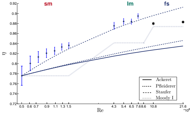
Figure 7. SCALE-UP AT \varphi/\varphi_{opt} = 1.1, \Delta\beta_s = 0^\circ
