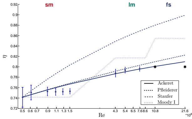
Figure 10. SCALE-UP AT \varphi/\varphi_{opt} = 0.85 , \Delta\beta_s = 0^\circ
