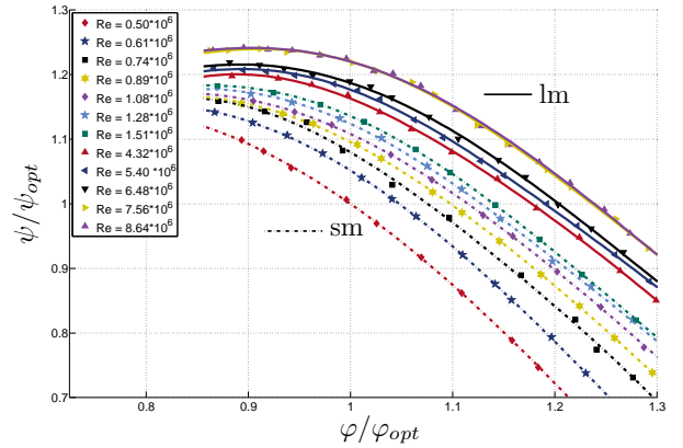
Figure 5. INCREASE OF TOTAL PRESSURE FOR DIFFERENT REYNOLDS-NUMBERS AND \varphi/\varphi_{opt} at \Delta\beta_s = -6^\circ
