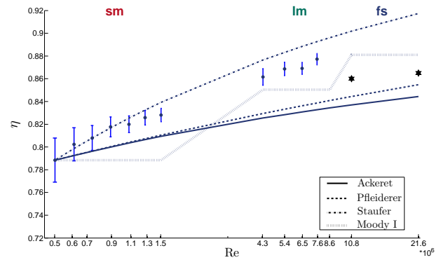
Figure 6. SCALE-UP AT \varphi/\varphi_{opt} = 1 , \Delta\beta_s = 0^\circ
