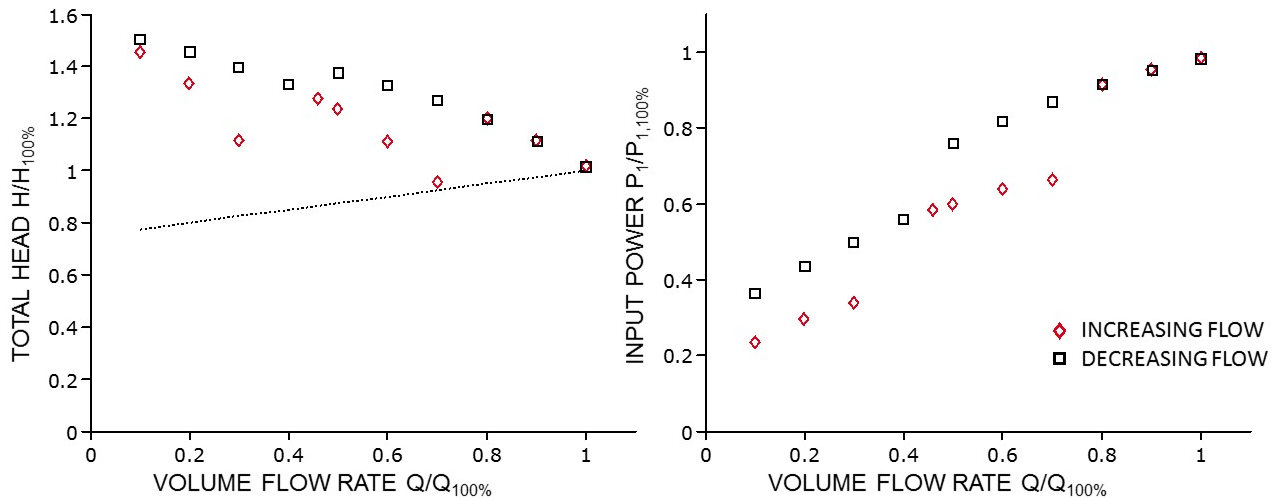
Figure 4: Comparison of total head and input power at the ten duty points at fixed speed mode of operation for increasing and decreasing flow rate.
