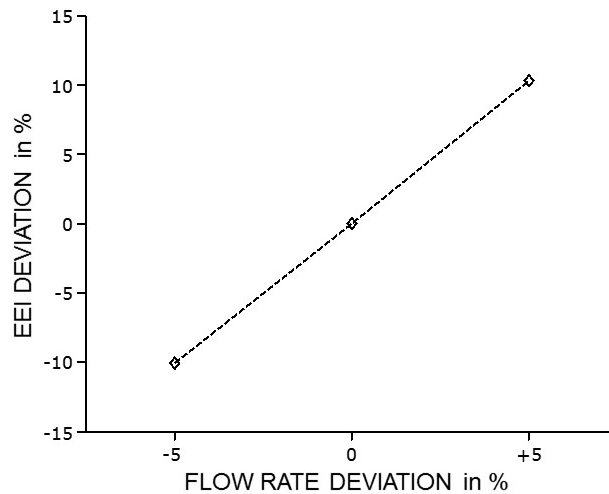
Figure 5: Influence of flow rate adjustment deviation on the EEI .
