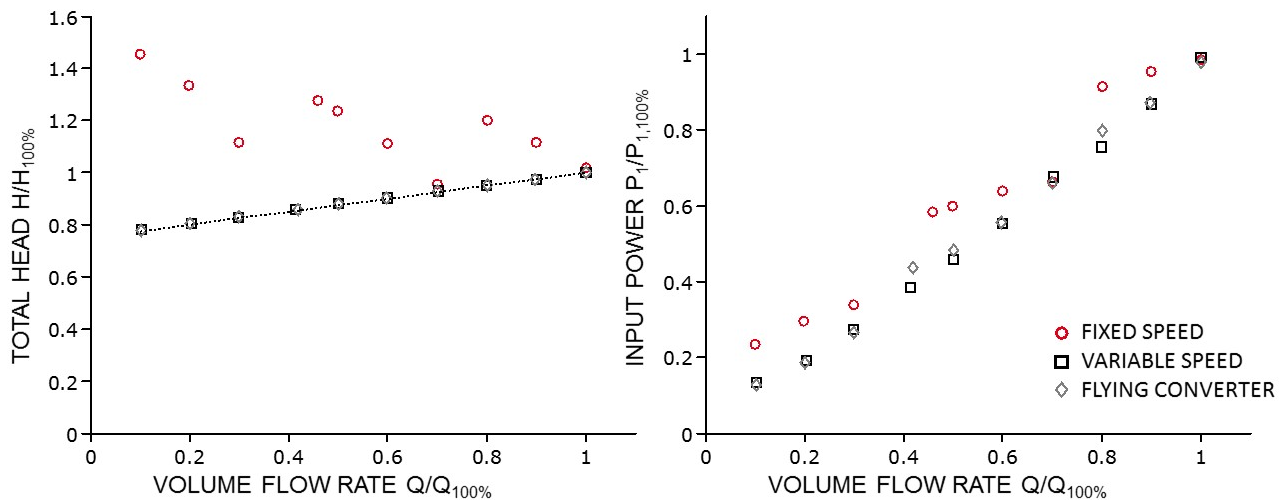
Figure 3: Comparison of total head and input power at the ten duty points at increasing flow rate for different modes of operation fixed speed, variable speed and flying converter.
