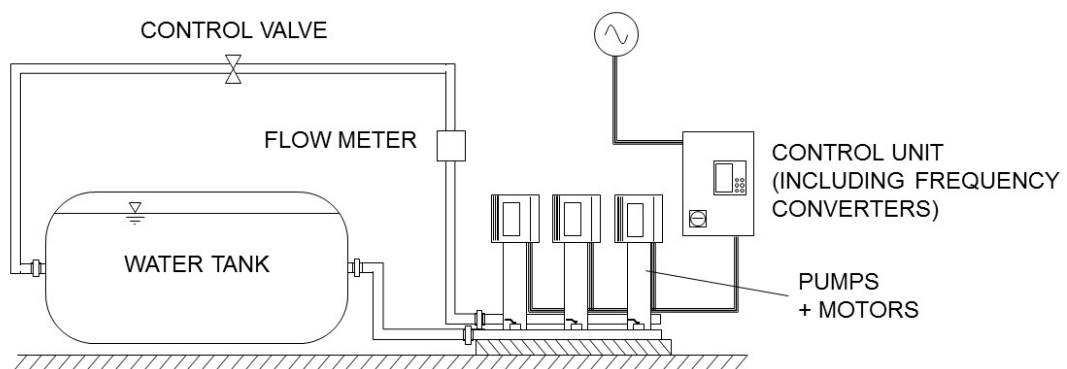
Figure 2: Experimental setup for EEI measurements at TU Darmstadt.
