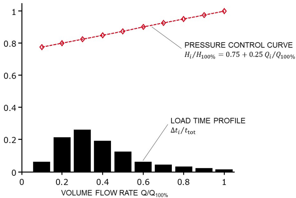
Figure 1: Standardized pressure control curve and load-time profile for booster pump units.
