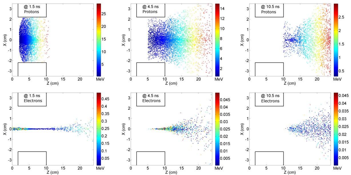
Figure 1. Snapshots of the proton (top) and electron (bottom) expansion for 3 different time steps: 1.5, 4.5 and 10.5 ns. Changing color scale for the particle energy because of better illustration, E_{p,max} = 29.5 MeV and E_{e,max} = 1.25 MeV.
