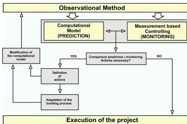
Figure 2. Observational method.
