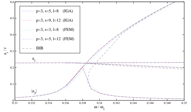
Fig. 19 Comparison of response curves for C^2 - (IGA) and C^1 -continuous (FEM) cubic B-Splines using HBNR
