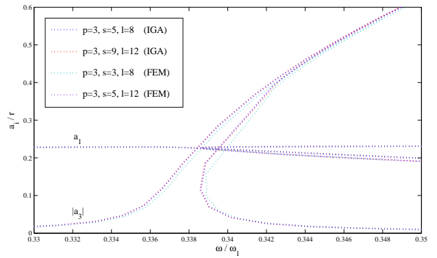
Fig. 20 Comparison of response curves for C^2 - (IGA) and C^1 -continuous (FEM) cubic B-Splines using IHB
