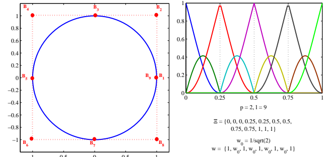
Fig. 3 A circle as a NURBS curve
