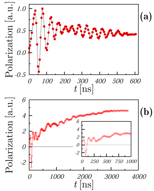
FIG. 7. Single pulse experiments on Ac-d 9 /Fl-d 8 h 2 in two different external fields \omega_n = \gamma_n \cdot B_{pol} . (a) \frac{\omega_{rf}}{2\pi} = 181 MHz = \frac{\omega_0}{2\pi} + \frac{\sigma_{EPR}}{2\pi} , \sqrt{2} \cdot \frac{\omega_1}{2\pi} = 23.5 MHz, \frac{\omega_n}{2\pi} = 2.0 MHz, T = 300 K. (b) \frac{\omega_{rf}}{2\pi} = 1.5 GHz = \frac{\omega_0}{2\pi} + \frac{\sigma_{EPR}}{2\pi} , \sqrt{2} \cdot \frac{\omega_1}{2\pi} = 9.3 MHz, \frac{\omega_n}{2\pi} = 4.2 MHz, T = 300 K.
