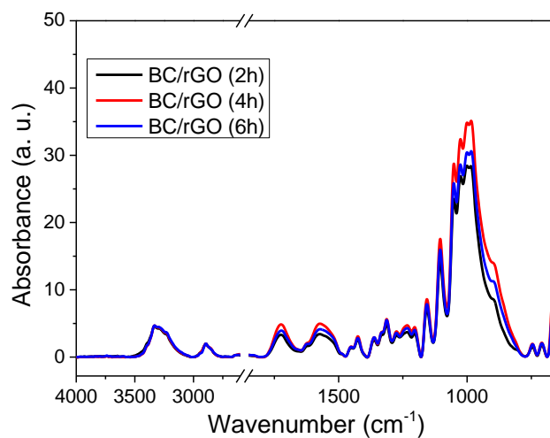
Figure S2. FT IR spectrum of BC/rGO after the reduction for 2, 4, and 6 h.
