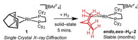
Scheme 3. Stable \sigma -Alkane Norbornane Complex, [\text{Rh}(\text{Cy}_2\text{PCH}_2\text{CH}_2\text{PCy}_2)(\eta^2,\eta^2\text{-C}_7\text{H}_{12})][\text{BAR}^{\text{F}}_4] , 2 , Formed from a Solid/Gas Single-Crystal to Single-Crystal Reaction between \text{H}_2 and Norbornadiene Precursor, 1 48
