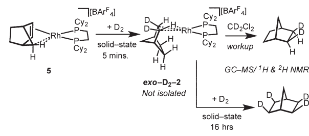
Scheme 8. Addition of D 2 to a Norbornene Precursor, 5
