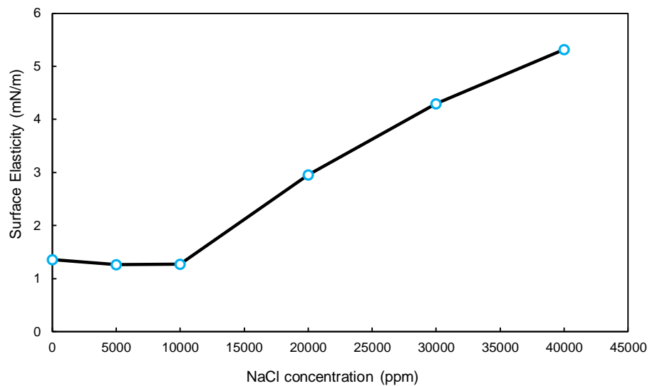
Figure S1. Surface elasticity values of aqueous solutions of 0.1 wt.% XG, 16.6 mM SDS for various concentrations of NaCl at a fixed frequency of 0.05 Hz
