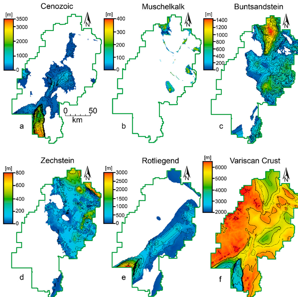
Figure S1. Maps of thicknesses of the six geological units from the top a: Cenozoic sediments, b: Muschelkalk, c: Buntsandstein, d: Zechstein, e: Rotliegend and f: the Variscan crust at the model base, down to a depth of 6 km below msl.
