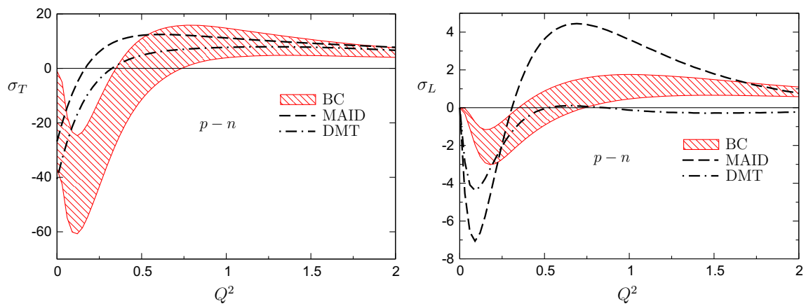
Fig. 2 Consistency check at the transition point W = 1.3 . The plot compares the representations of MAID and DMT used below that point with the BC-parameterisation used above it. The difference between MAID and DMT and the band attached to BC represent an estimate
