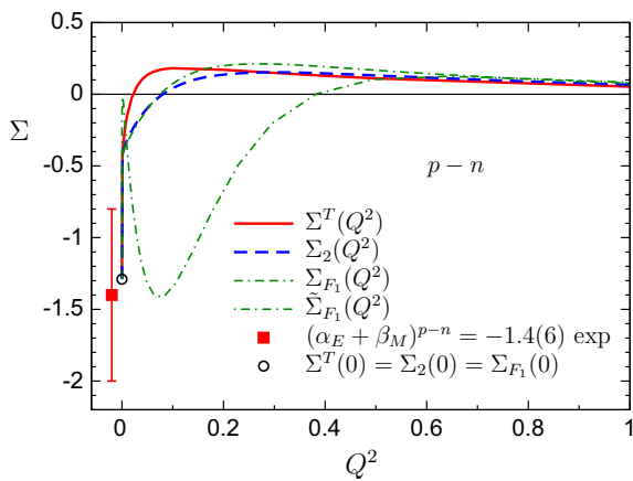
Fig. 5 Cross section integrals relevant for the difference between proton and neutron
